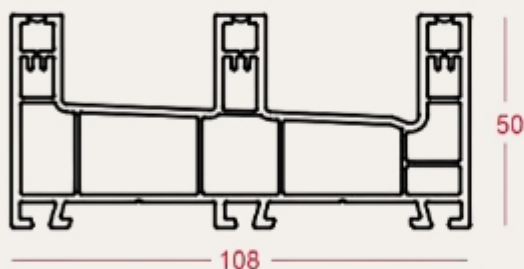
Sliding Frame 3 Track SBM-SS-003
