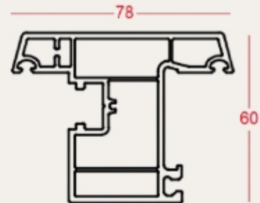
Casement Outward Sash 60mm SBM-CS-002
