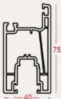
Sliding Sash 75mm SBM-SS-005
