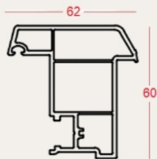
Casement Fly Mullion 60mm SBM-CS-009
