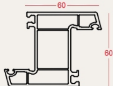
Casement Z Mullion 60mm SBM-CS-008
