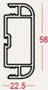
Mosquito Mullion SBM-SS-009
