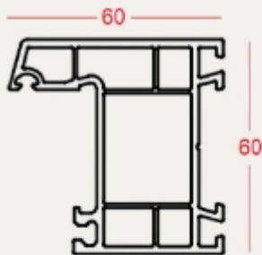
Casement Frame 60mm SBM-CS-001
