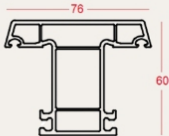
Casement T Mullion 60mm SBM-CS-007
