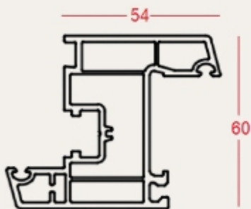
Casement Inward Sash 60mm SBM-CS-003
