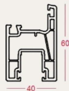
Sliding Sash 60mm SBM-SS-004
