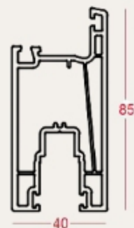
Sliding Sash 85mm SBM-SS-006
