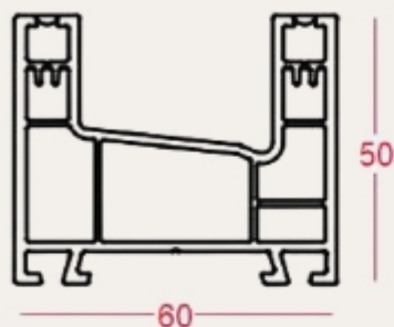
Sliding Frame 2 Track SBM-SS-001
