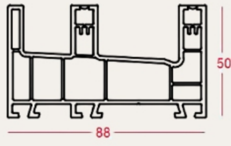
Sliding Frame 2.5 Track SBM-SS-002
