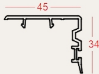
Interlock SBM-SS-010
